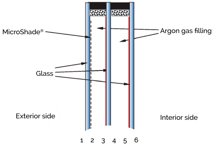
Figure 2. A glazing composition of a 3-layer LowE glazing with MicroShade®. The numbers indicate the indexing of the glazing surfaces.
