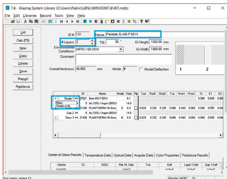
Figure 7: Example of a 3-layer MicroShade® glazing. Please note the position of the low-e coating on side 3 and 5. The blue areas indicate where to change the name, the amount of layers and the first layer to a "Shade or frit".
